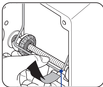
End-stop spring
